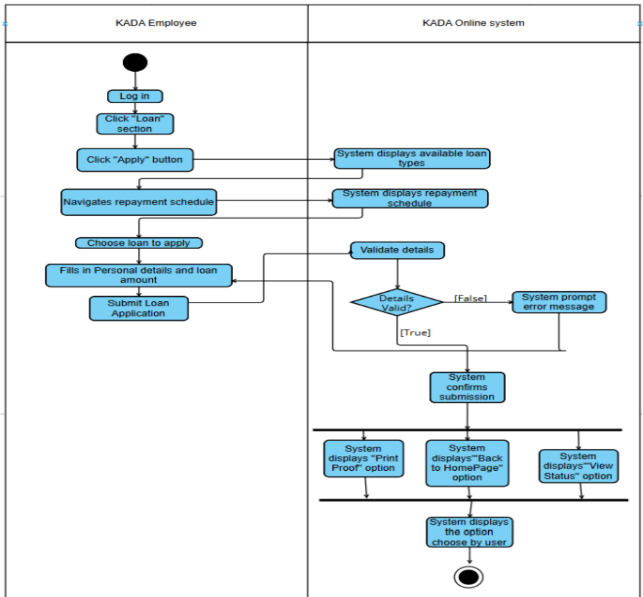
Figure 4.2.4 UC04: Apply Loan
