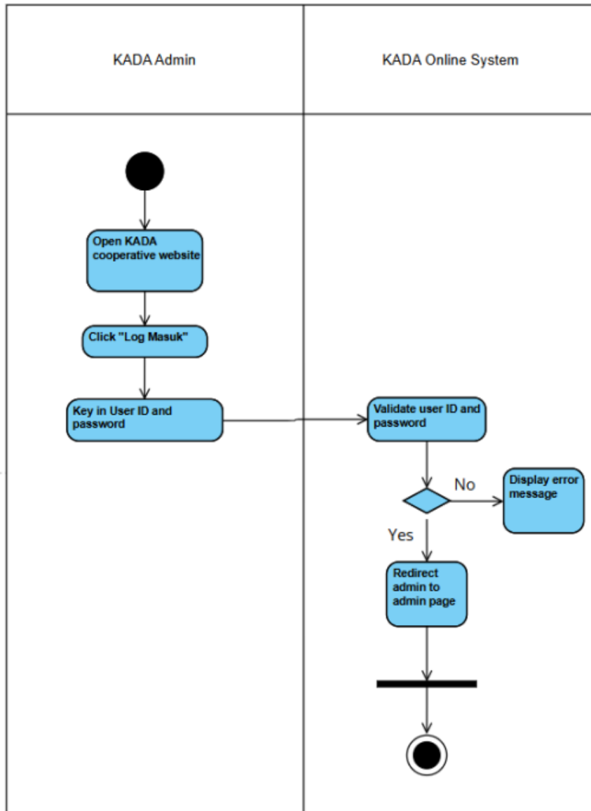
Figure 4.2.3 UC03: Log in (Admin)
