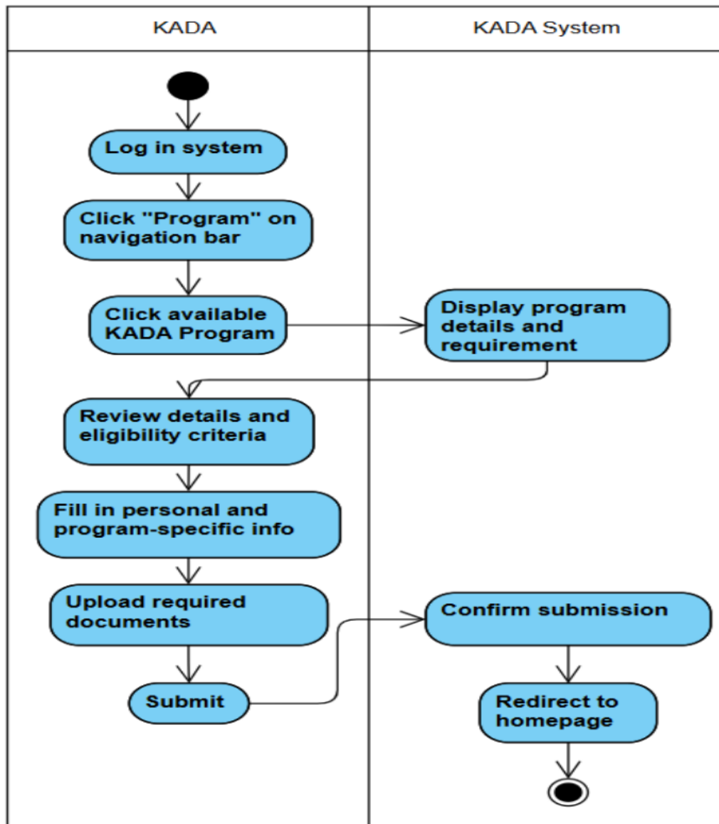
Figure 4.2.5 UC05: Apply Program
