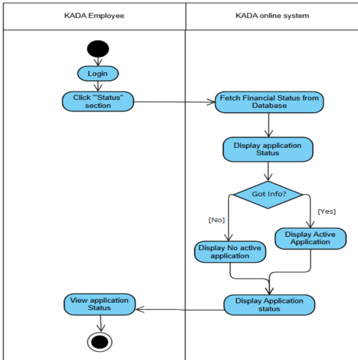
Figure 4.2.2 UC02: View Application Status
