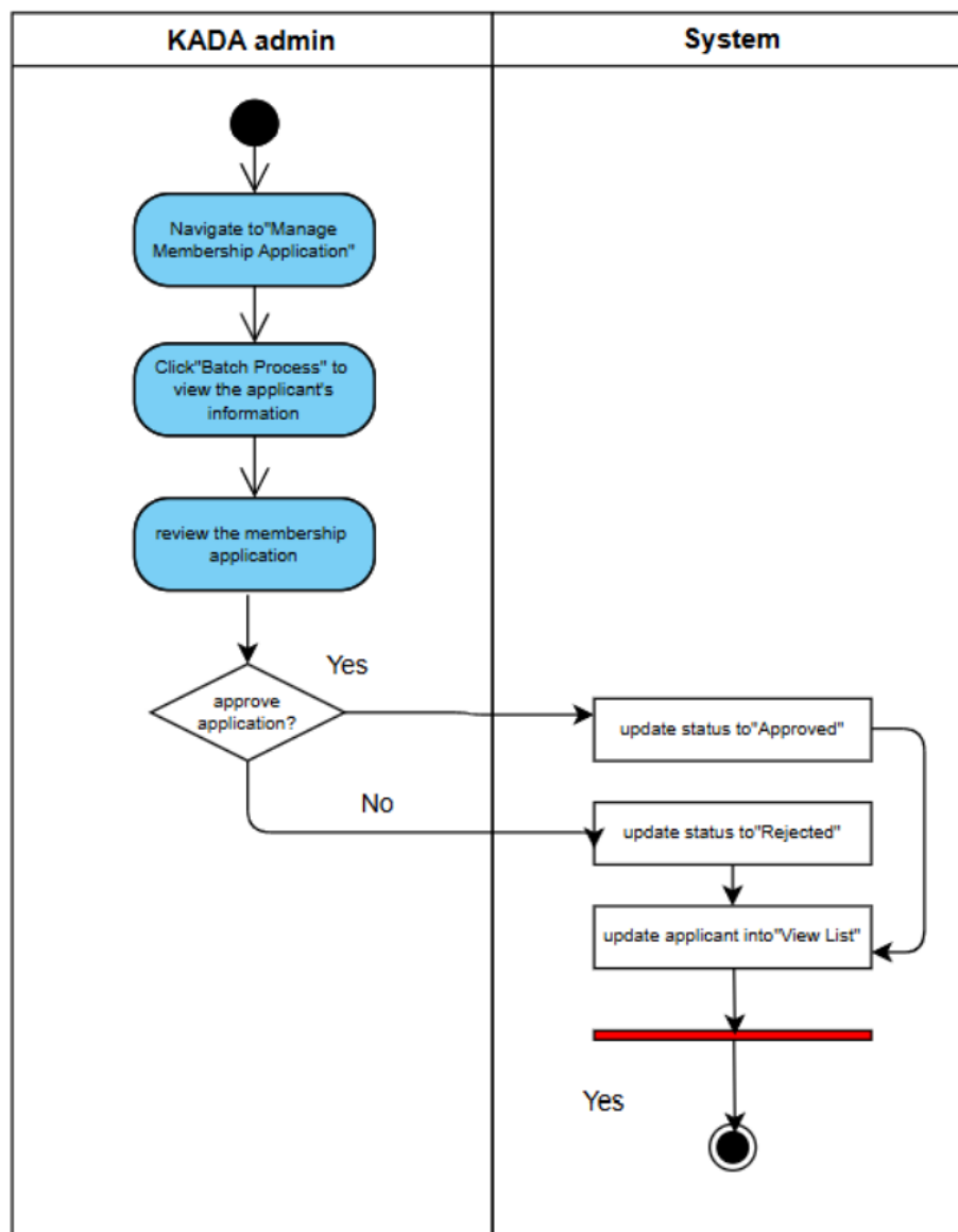
Figure 4.2.10 UC10: Approve Membership Application
