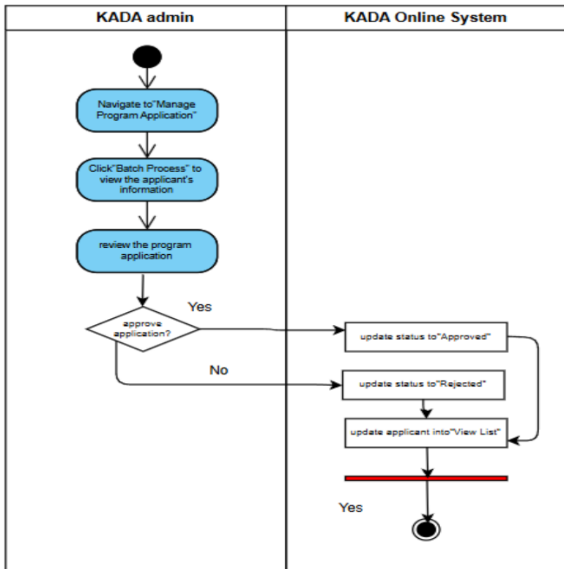
Figure 4.2.12 UC12: Approve Program Application
