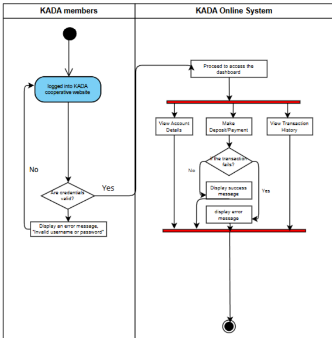
Figure 4.2.6 UC06: Manage Savings Account
