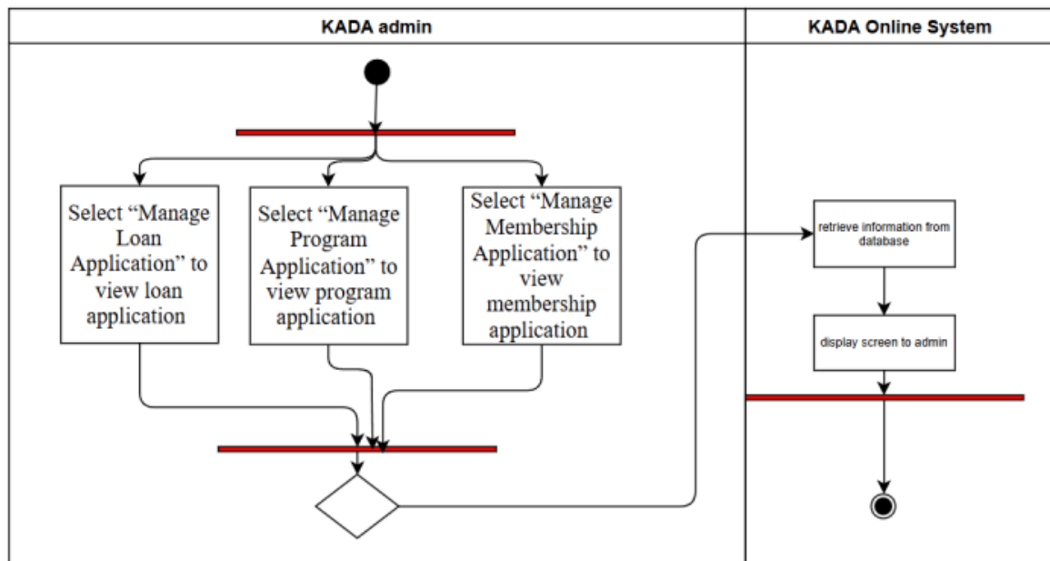
Figure 4.2.9 UC09: Admin View Application List
