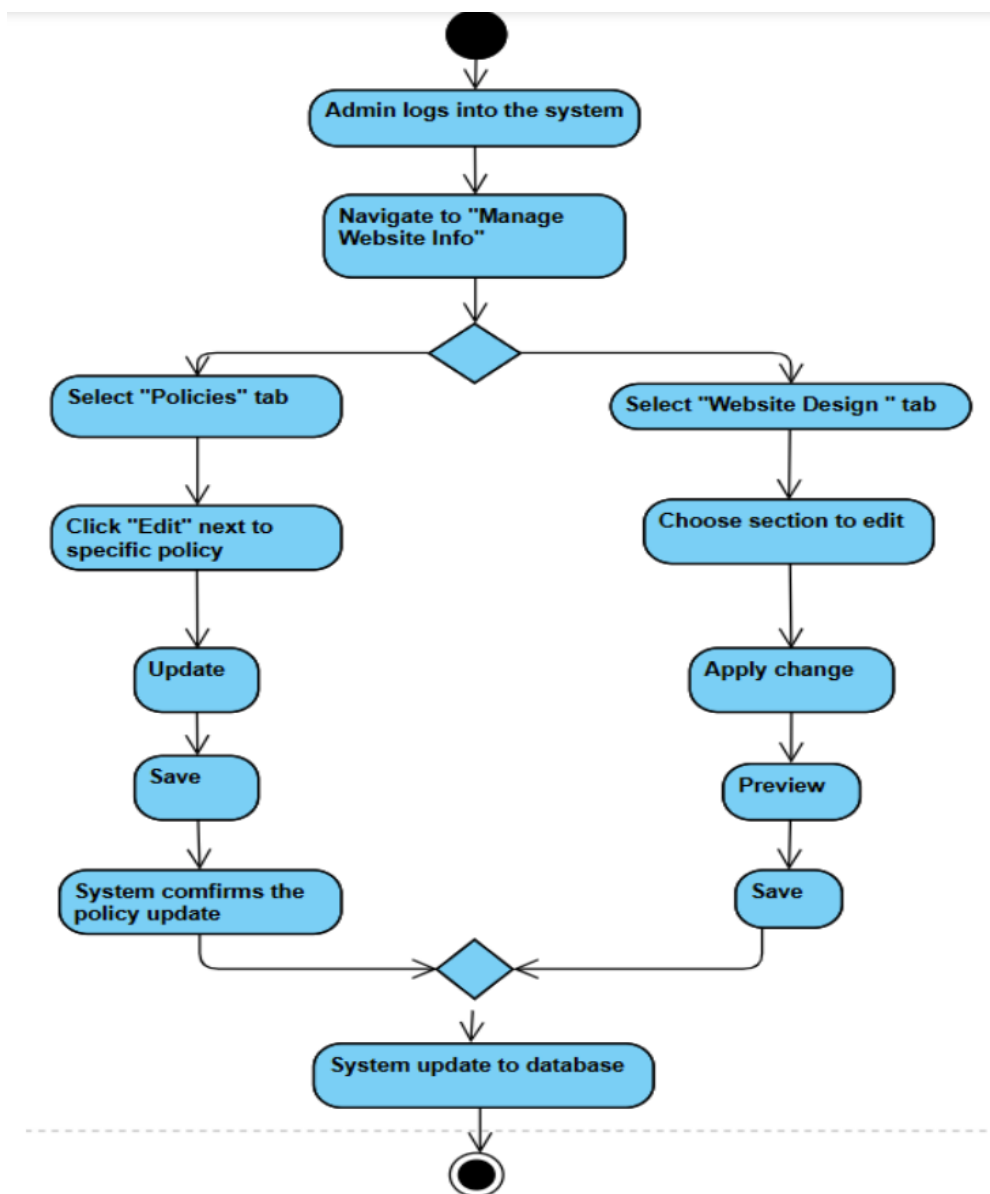
Figure 4.2.13 UC13: Manage Website
