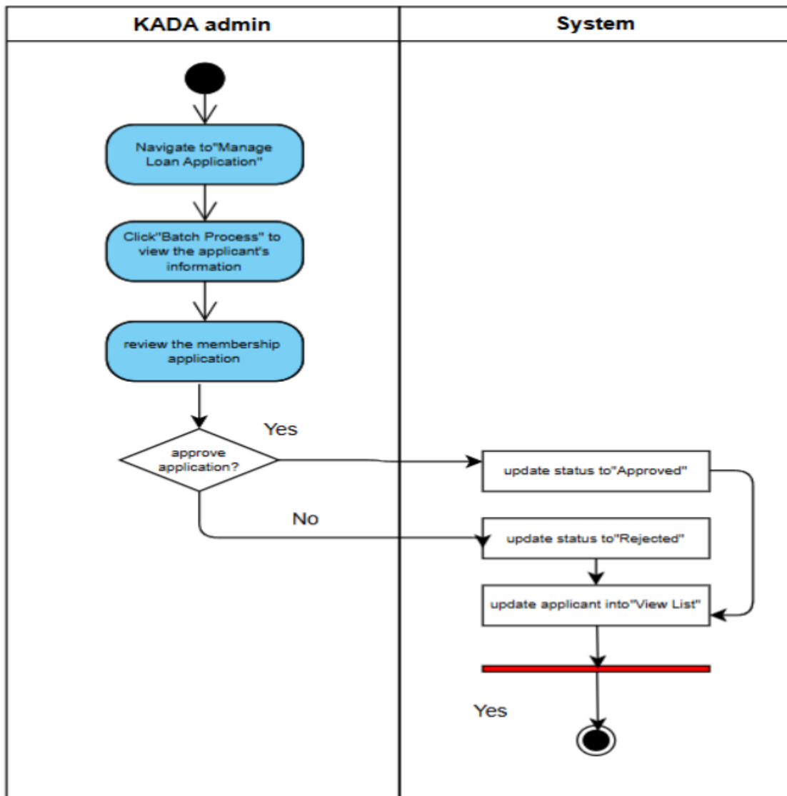
Figure 4.2.11 UC11: Approve Loan Application
